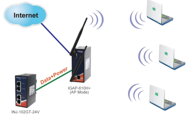
AP Mode
